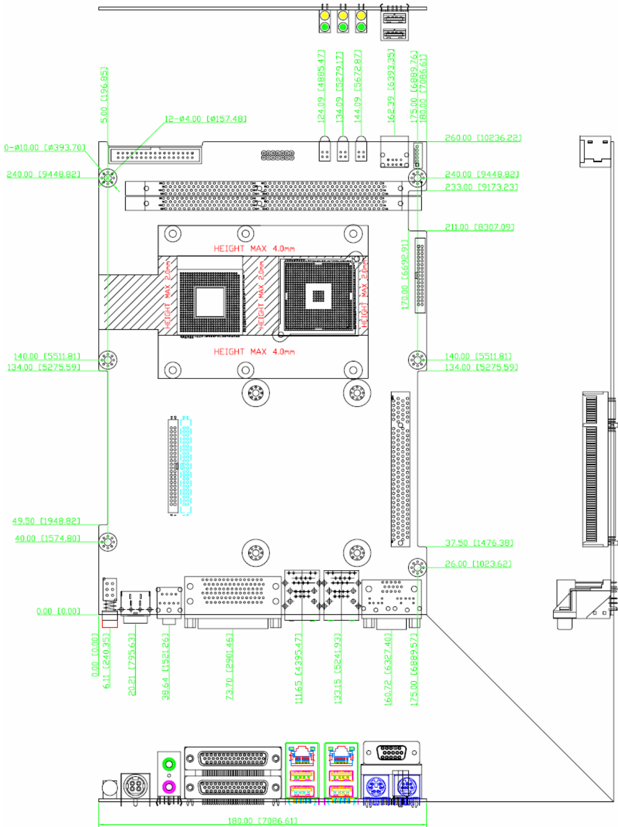
Figure 1.2: Mechanical Drawing of the EBC573
