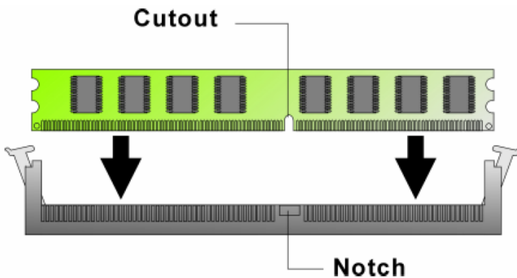
Figure 3-2: How to Install DIMM (2)
