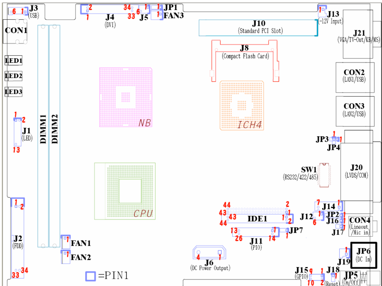
Figure 2-1: Jumper Location
