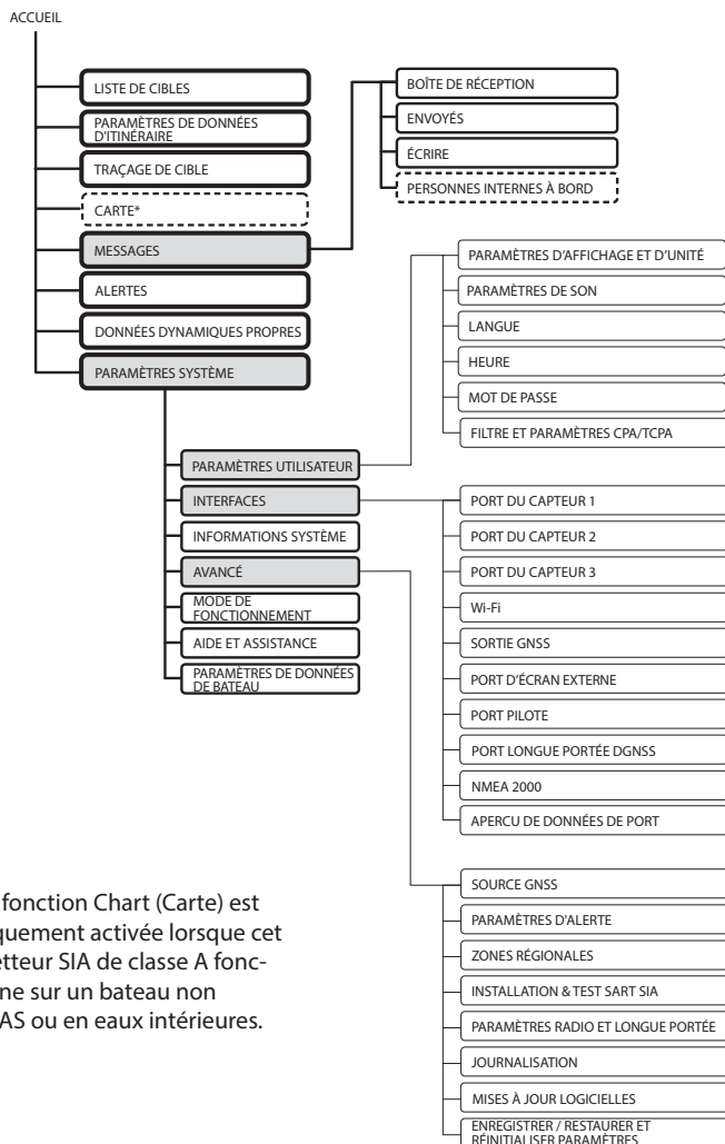
Figure 20 Structure du menu principal
