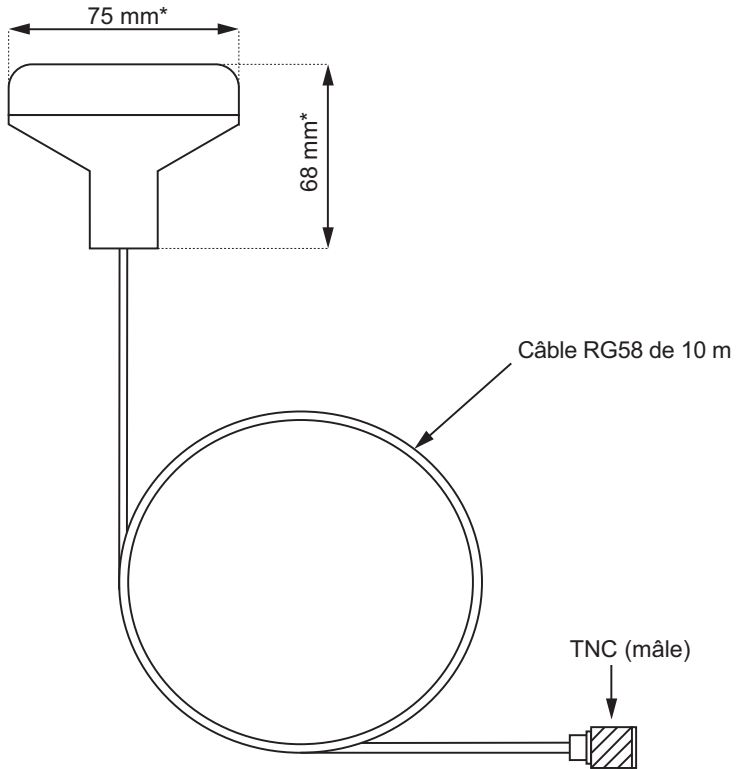
Figure 32 Antenne GNSS
