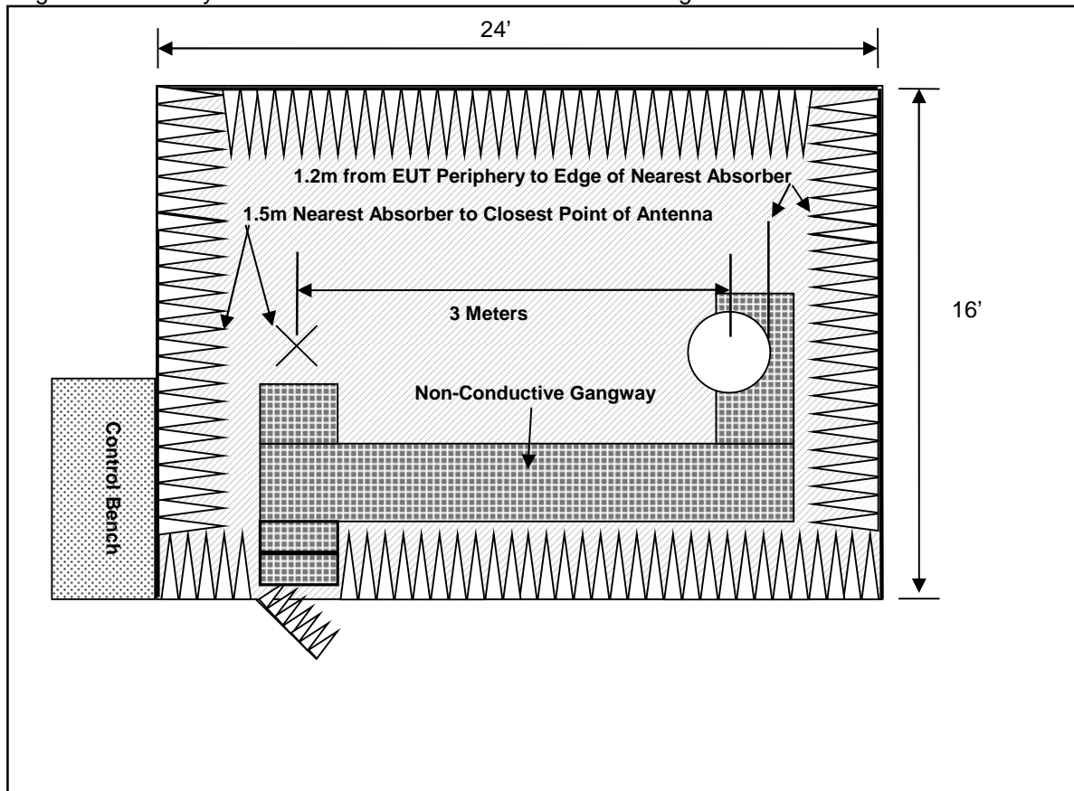
Figure 4.1.1.3-1: Fully Anechoic Chamber Test Site
