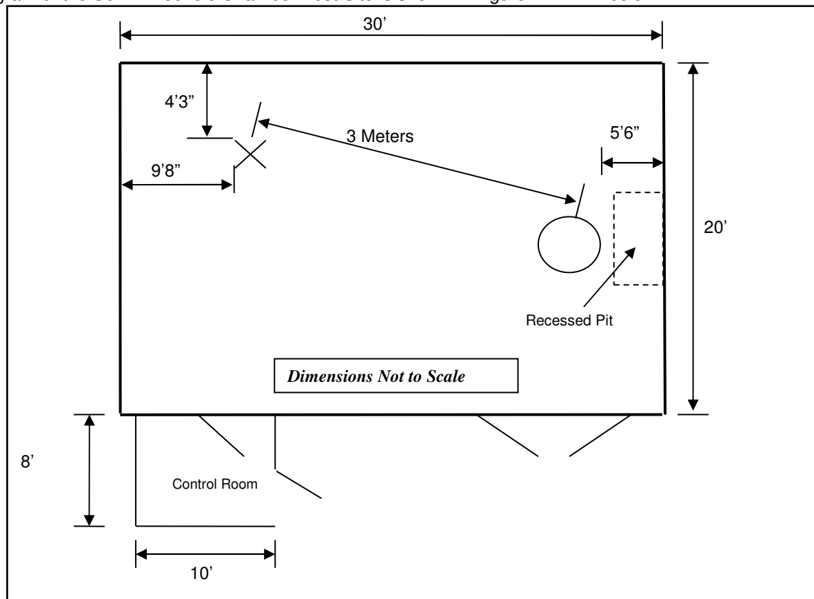
Figure 4.1.1.2-1: Semi-Anechoic Chamber Test Site
