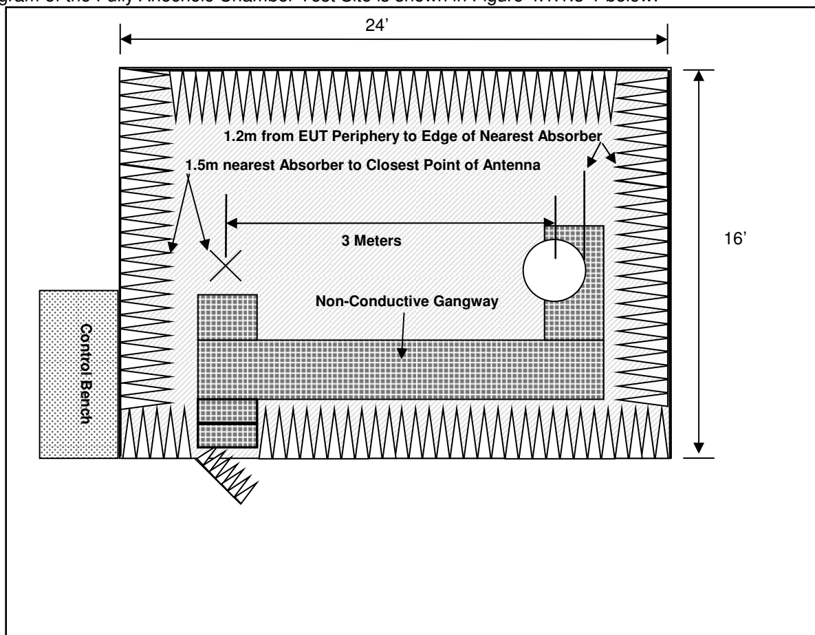
Figure 4.1.1.3-1: Fully Anechoic Chamber Test Site
