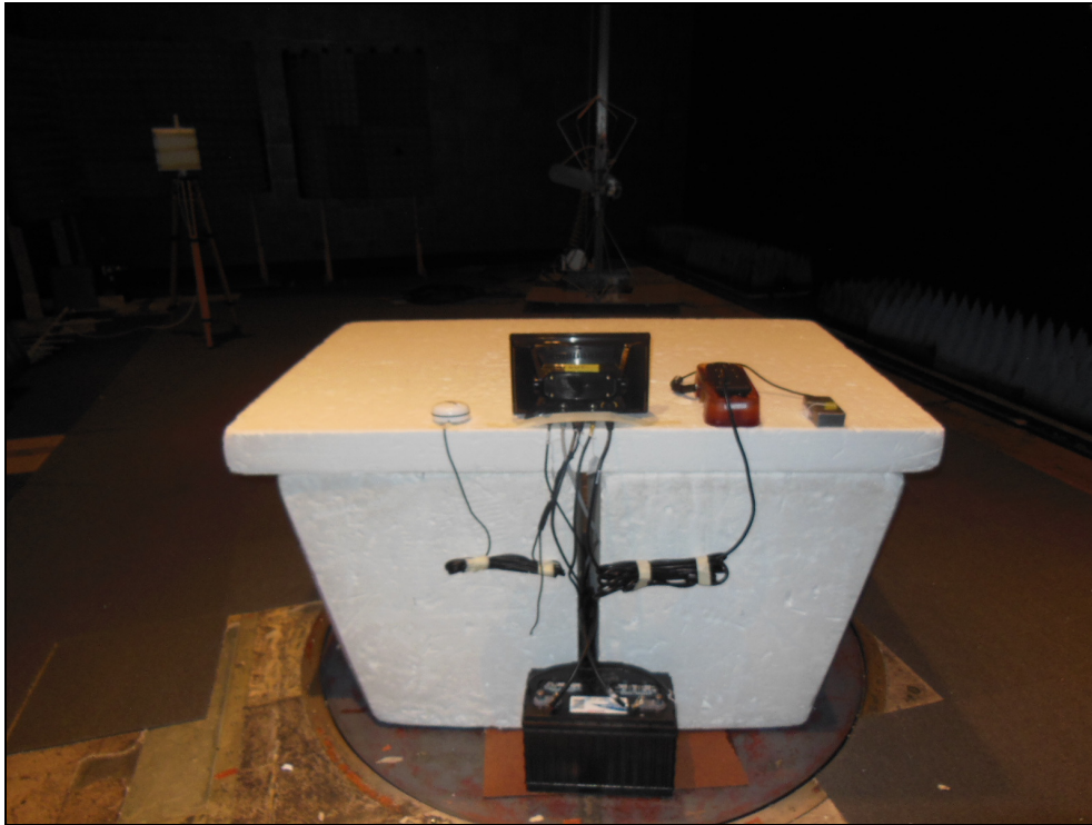
Figure 4.1.4-2: Radiated Emissions - Rear View - SAC
