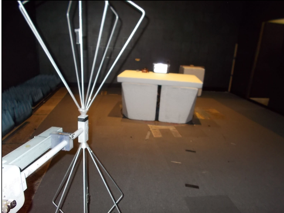
Figure 4.1.4-3: Radiated Emissions – Front View – Above 30MHz
