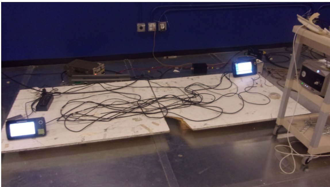
Figure 8.4-1: Test Setup Photograph
