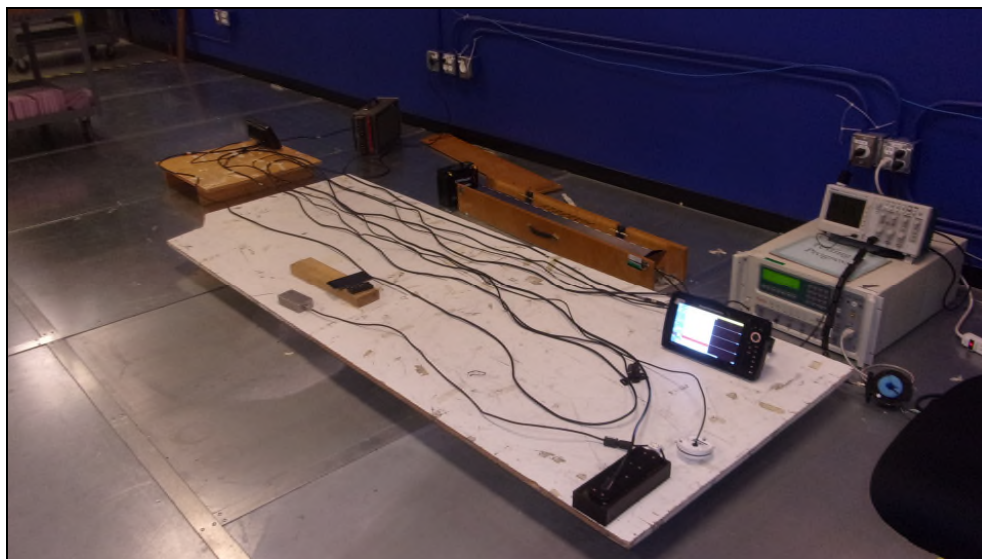
Figure 6.4-1: Test Setup Photograph
