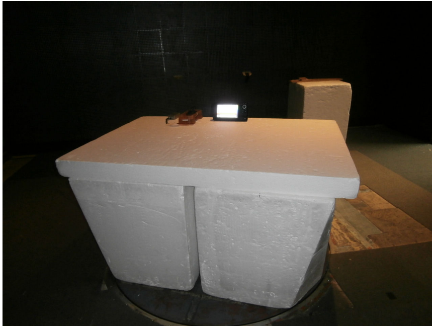
Figure 4.1.4-1: Radiated Emissions - Front View
