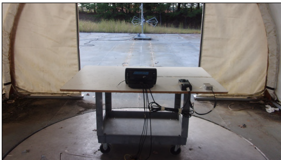
Figure 4.1.4-2: Radiated Emissions - Rear View
