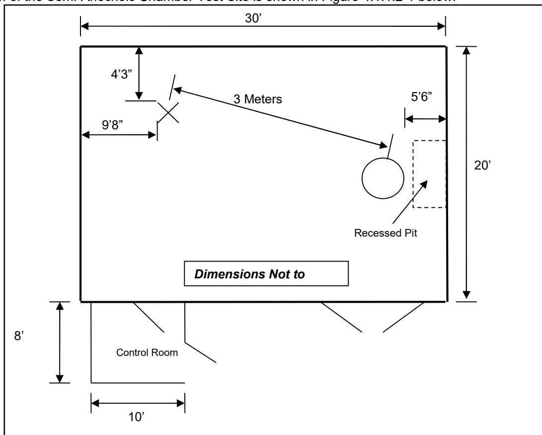
Figure 4.1.1.2-1: Semi-Anechoic Chamber Test Site
