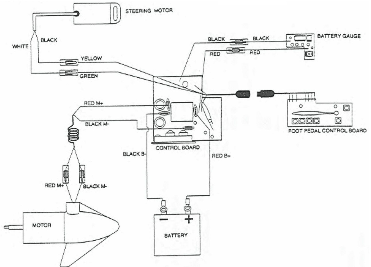
Wiring Diagram
