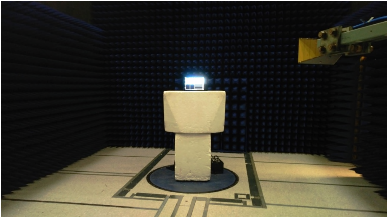
Figure 9-3: Radiated Emissions Test Setup
