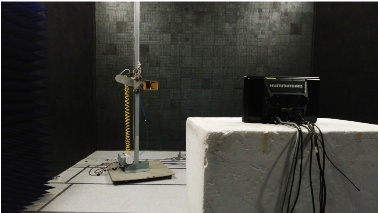
Figure 9-4: Radiated Emissions Test Setup
